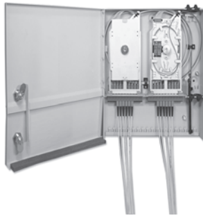
24-fibre capacity box (open)
