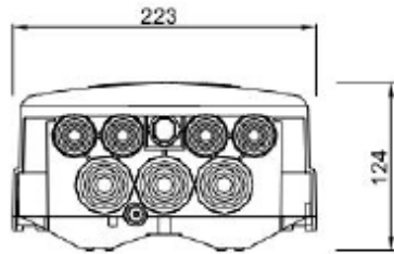
Underside View
