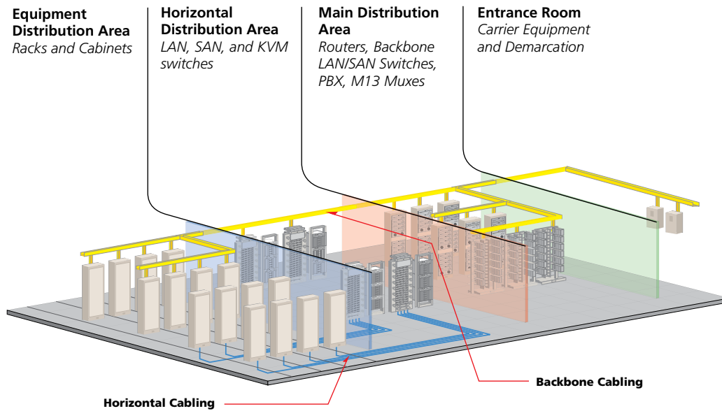
Data Centre according to TIA-942
