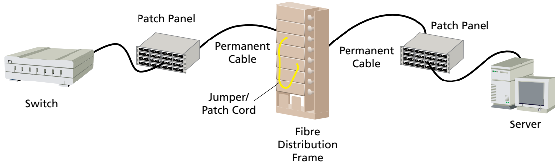
Cross-Connect Diagram, best versatile solution
